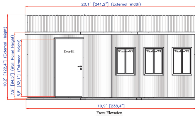
20 Ft x 8.5 Ft Tiny House Complete Building Dimensions
