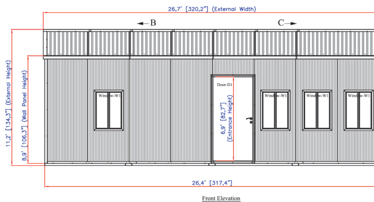
26 Ft x 8.5 Ft Tiny House Complete Building Dimensions
